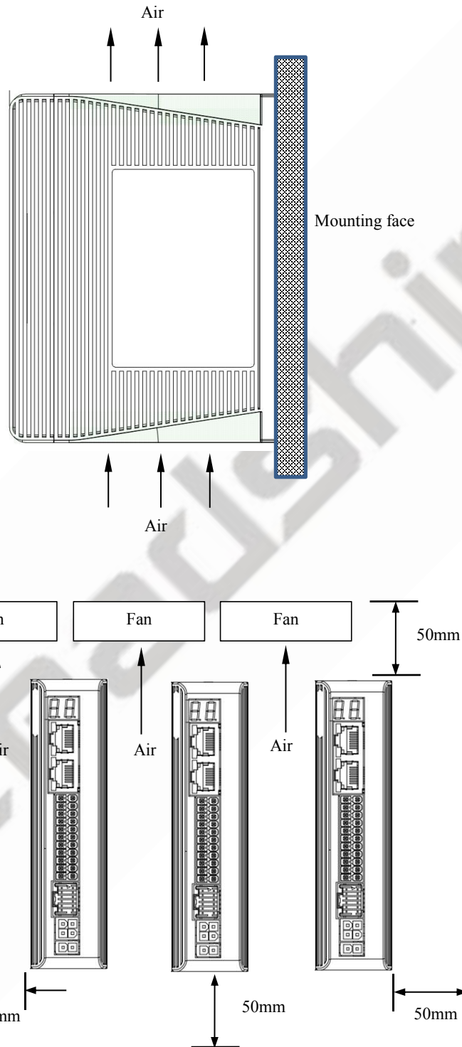
Figure 2.2: CS3E series installation drawing
