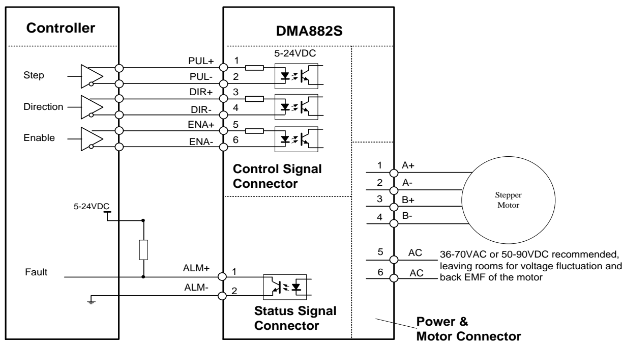
Figure 10: Typical connection
