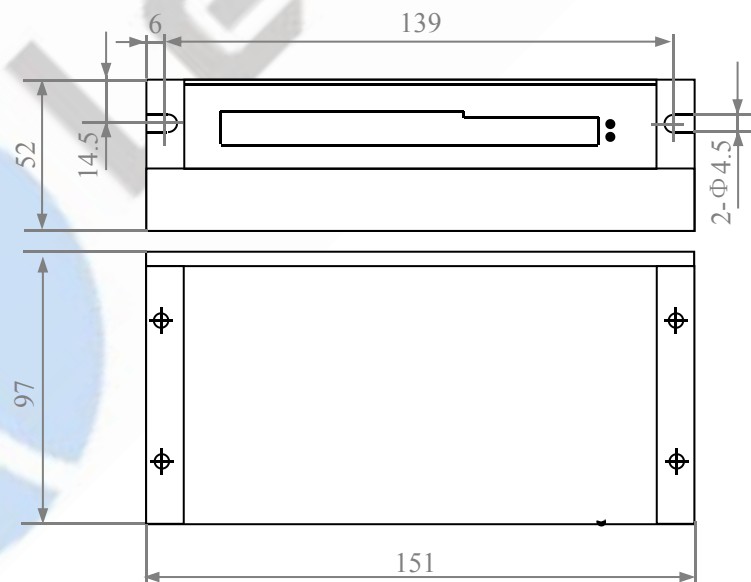
Figure 1 Mechanical specifications
