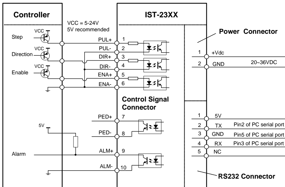
Connect IST-23XX to controller of sourcing output
