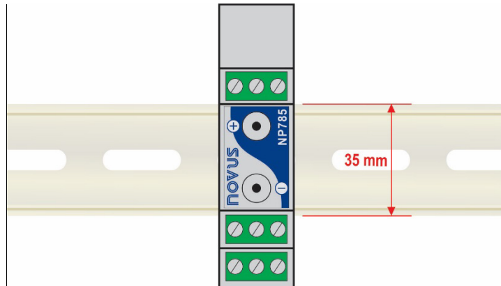
Figure 2 – Mechanical installation
