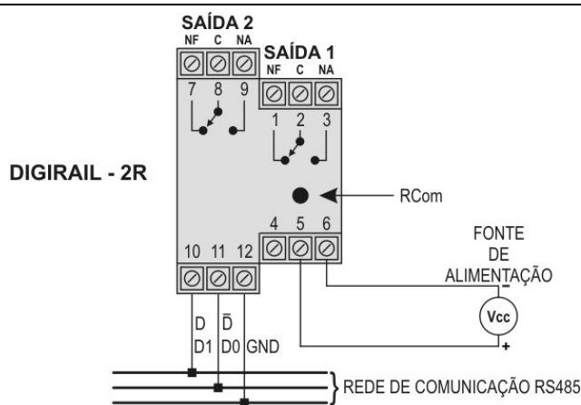
Figure 2 – Electrical Connections
