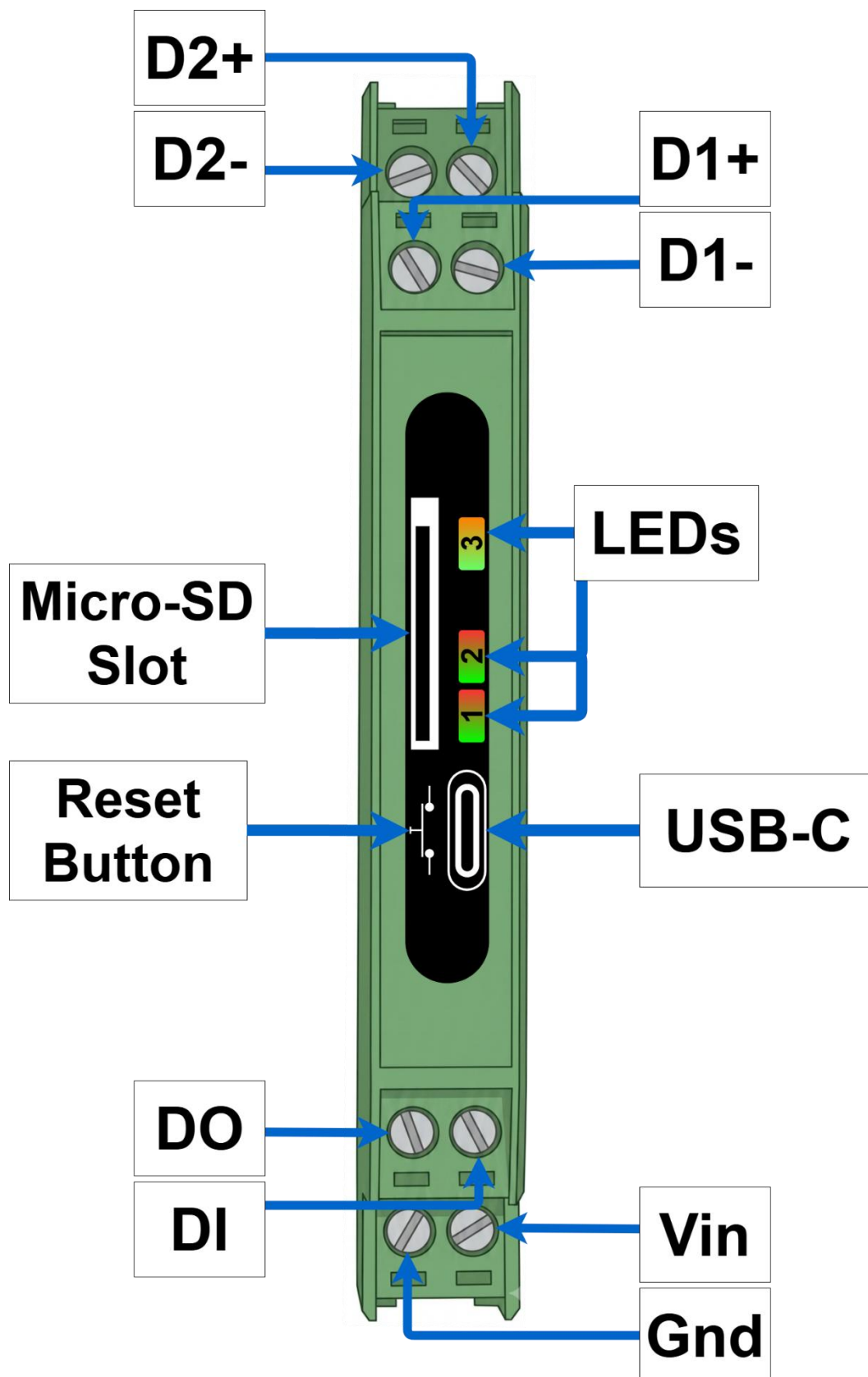
Figure 5: Connection/Peripherals Diagram
