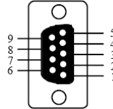
DB9F (Female/hole)
