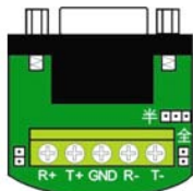
DB9F to 5 bit terminal block
