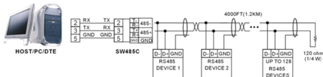
Figure 2: Master/Slave multi-drop configuration in RS485 mode
