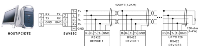
Figure 4: Master/Slave multi-drop configuration in RS422 mode
